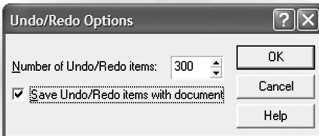
Figure 2. Undo/Redo Options.
