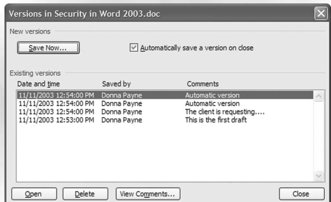
Figure 7. Microsoft Versions.
